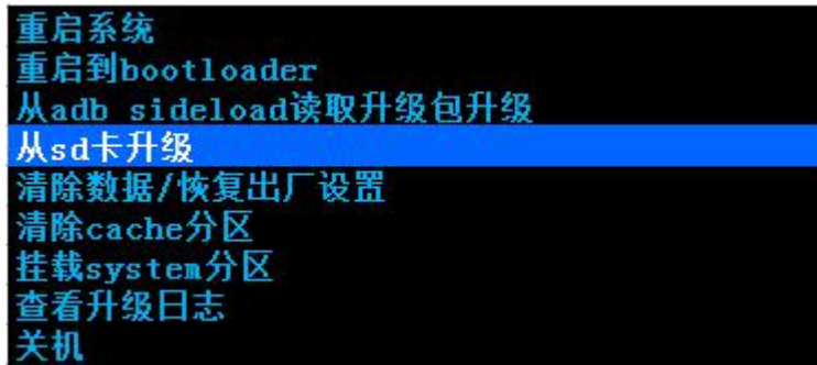
图 3-2 Recovery 菜单
