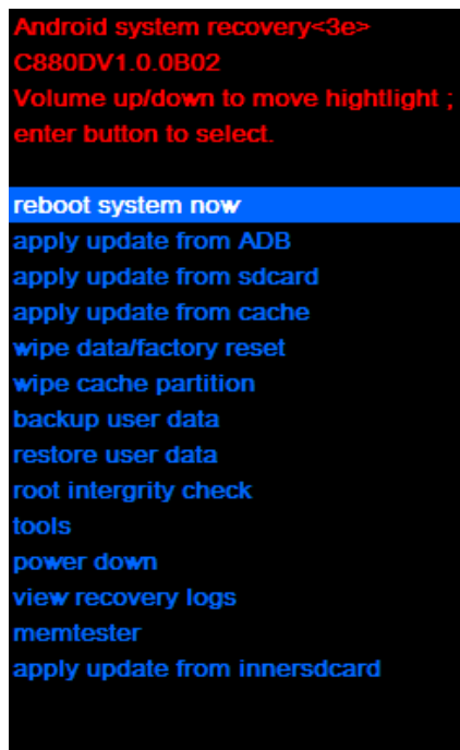
图 3-4 Recovery 菜单
